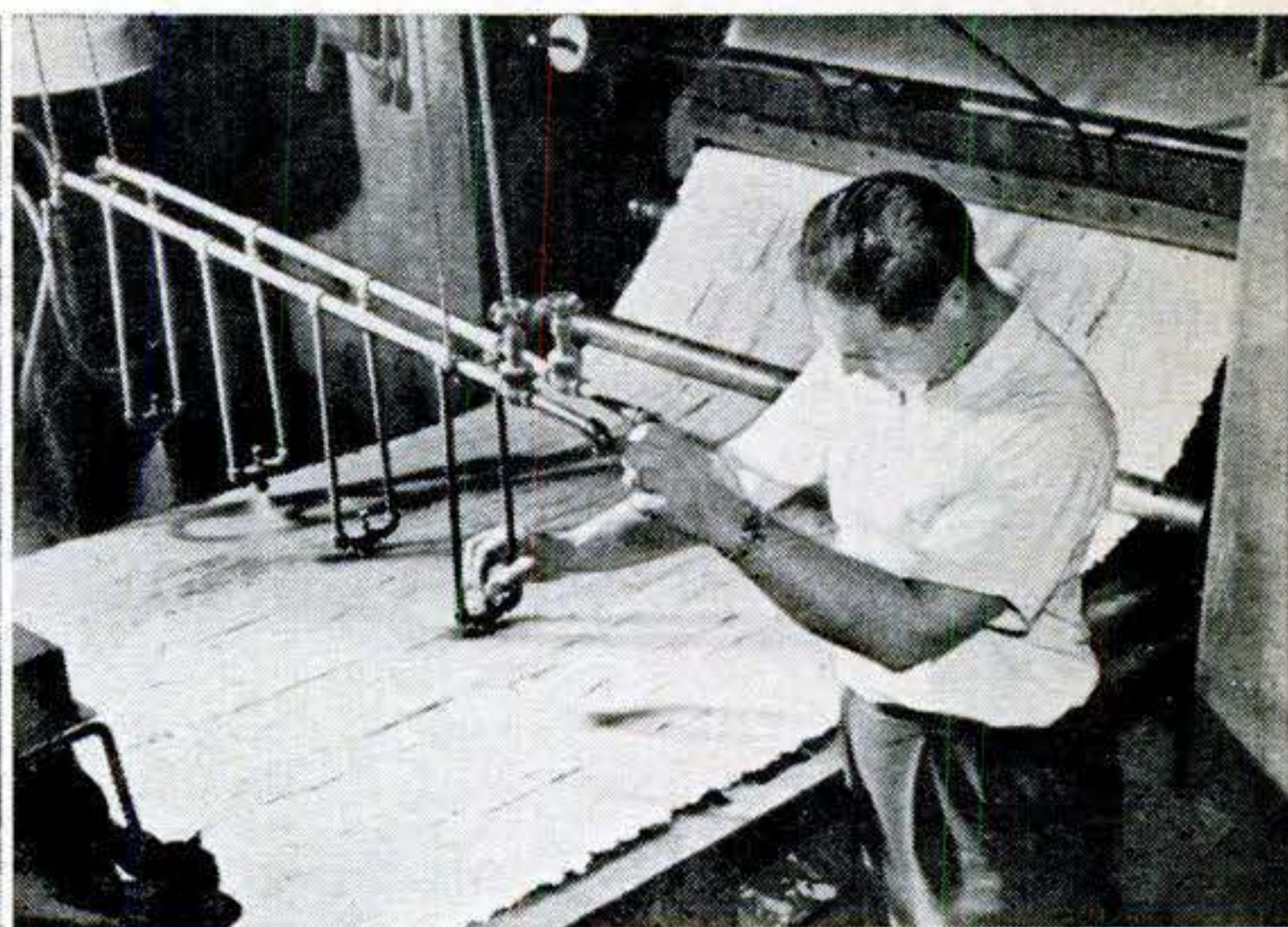
4 THE SHEET , after going through a calendering operation, has been reduced to either of two thicknesses— \frac{1}{8} inch or \frac{3}{16} inch. Here an operator is adjusting wax sprays. The sheet also passes under cooling sprays and polishing buffer.
